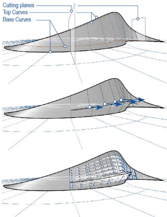
Figure 2: The top image denotes the placement of cutting planes which divide it into manageable pieces. The middle piece can then form deviations for seating seen in the middle image. The bottom image shows how the reinforcing pattern for formwork is incorporated into the design logic.
